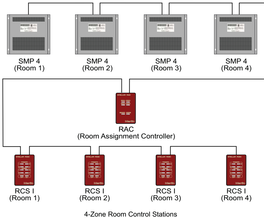
Four Stellar Mini Panels for four partitioned spaces, with RAC room assignment controller, and four RCS I four-preset/four-zone room control stations
