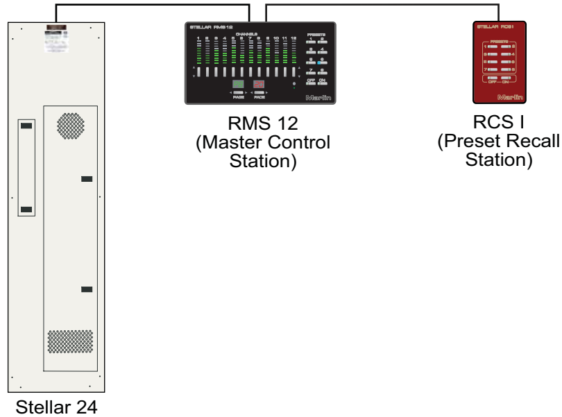
Stellar dimmer panel with 24 dimmers, RMS 12 master control station, and RCS I eight-preset remote recall station
