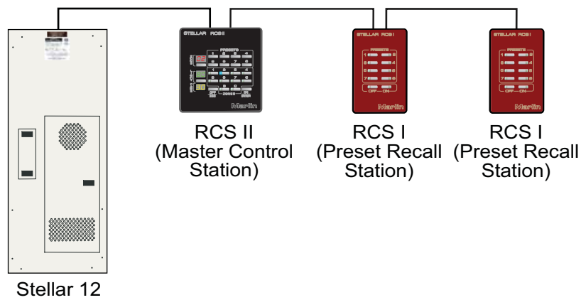
Stellar dimmer panel with 12 dimmers, RCS II master control station, and two RCS I eight-preset remote recall stations
